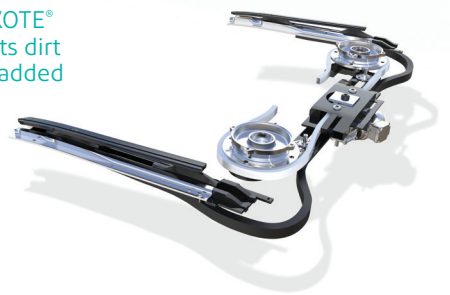
Typical lubrication points for sliding-roof designs, including sunroofs and panoramic roofs.
