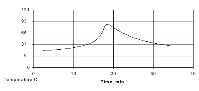
Typical Exotherm Curve for MA3940 at 23°C (10 grams) 5
