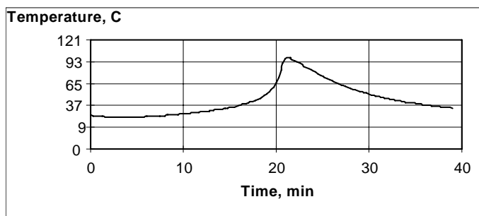
Typical Exotherm Curve for MA320 at 23°C (10 grams) 5
